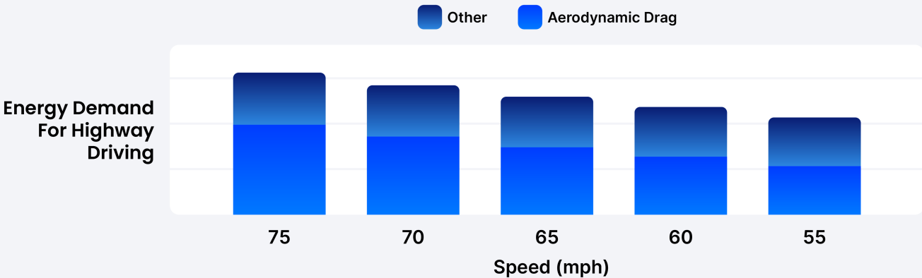
Figure 5: Highway driving energy demand vs. speed.
